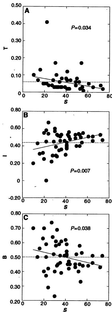
Fig. 1. Fraction of species in (A) top, (B) intermediate, and (C) basal categories as a function of S. Horizontal dashed lines represent scale-invariant estimates from (1). The simple least squares regressions, shown as solid lines, suggest that (fractions converted to percentages) T = -0.107S + 10 ( SE_{\text{slope}} = 0.057 , R^2 = 0.07 ), I = 0.284S + 33 ( SE_{\text{slope}} = 0.110 , R^2 = 0.12 ), and B = -0.177S + 57 ( SE_{\text{slope}} = 0.098 , R^2 = 0.06 ).
