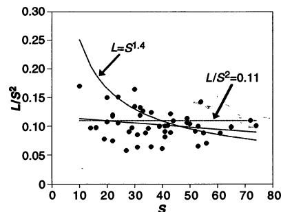
Fig. 2. Variation of directed connectance [ L/S^2 , (4)] with S. The simple least squares regression [Havens' estimate (1)], shown as a solid line ( L/S^2 = -0.00037S + 0.117 , SE_{\text{slope}} = 0.00024 , R^2 = 0.05 ), is not significantly different from the constant connectance hypothesis [ L/S^2 = 0.11 (4)] at P = 0.129 . Havens estimated (1) that L = S^{1.4} .
